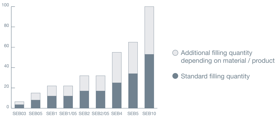
Conveying performance in m 3 /h
